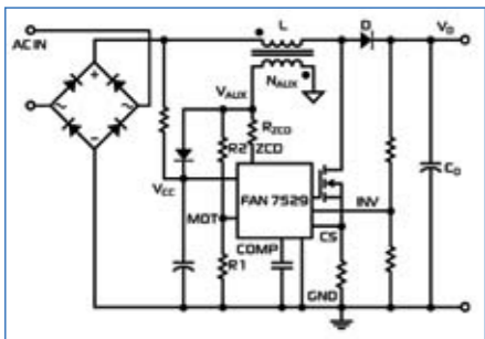
Figure 4: Typical application diagram for voltage mode control of transition mode PFC.
