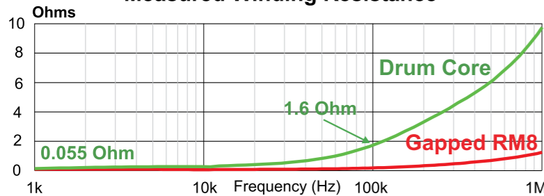
Figure 7: Measured winding resistance of a custom RM8 inductor design, and an off-the-shelf drum-core design.
