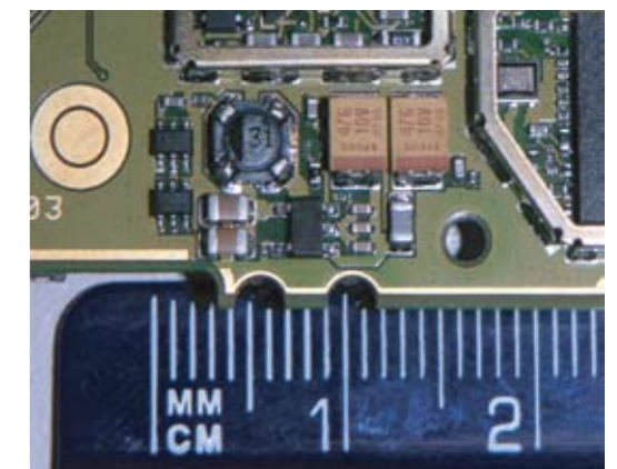
Figure 4: Industry standard SOT-23-5 buck regulator with winding coil inductor and large tantalum capacitor. The complete solution size is just ~140mm 2 .
