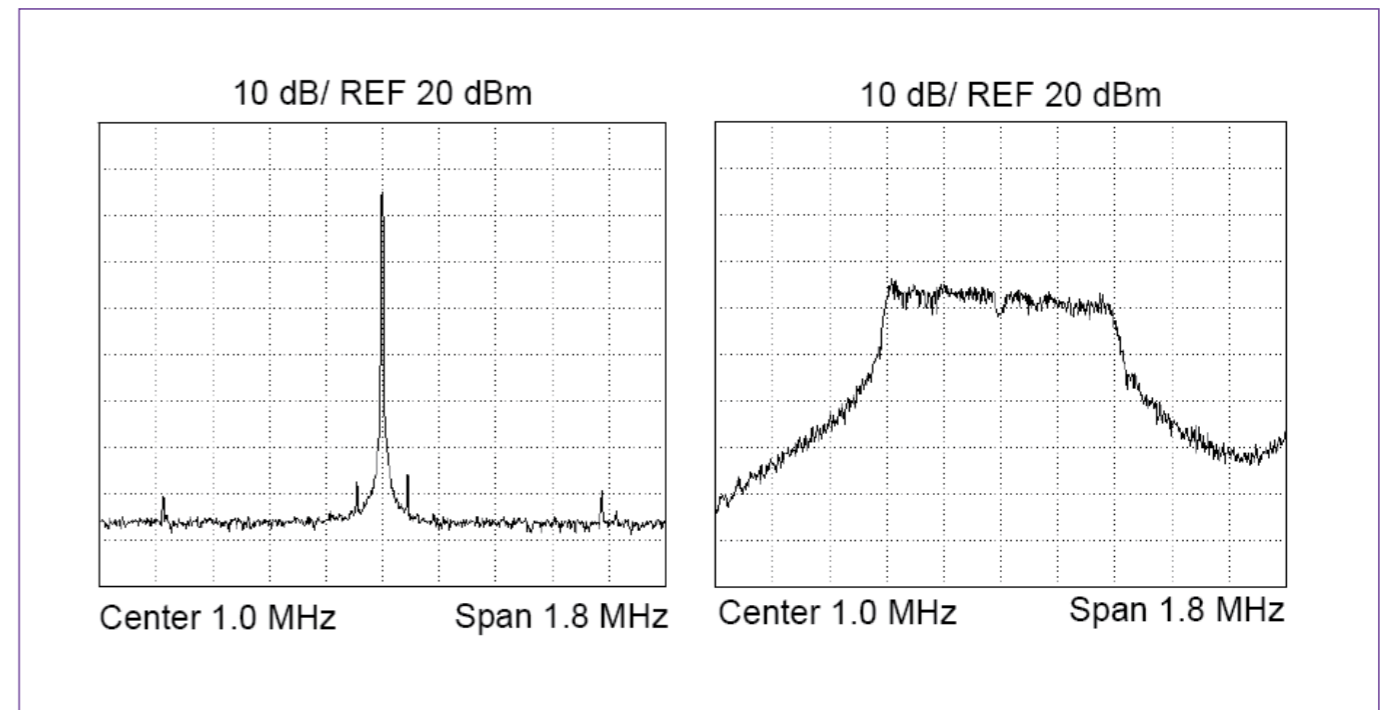
Figure 3. Spectrum of the Clock Output Before and After Dithering.
