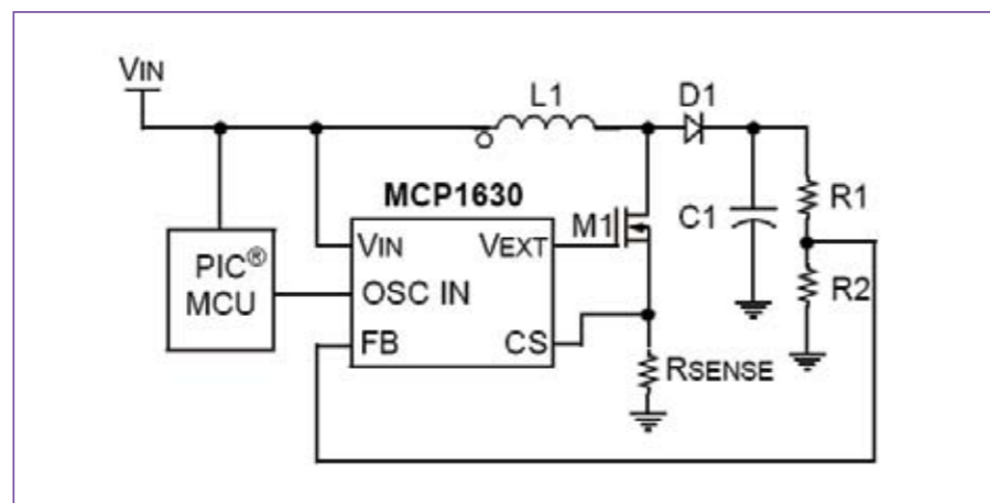
Figure 2. Using a PIC® Microcontroller as a Clock Source for a Booster Circuit.
